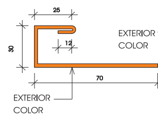
FRAMED OPENING TRIM
