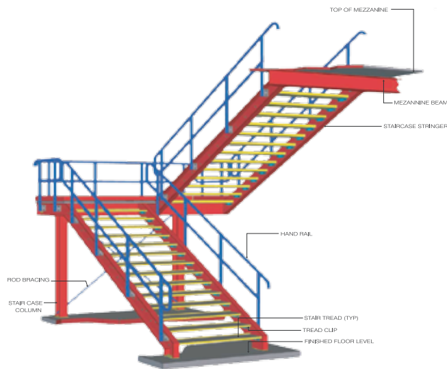
DOUBLE FLIGHT STAIRCASE WITH STAIR COLUMN FROM FFL
