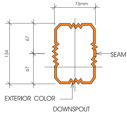
DOWNSPOUT
