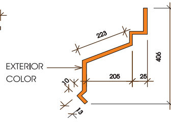
HOOD TRIM FOR SLIDING DOOR
