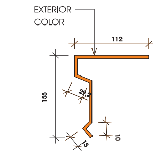
OASIS EAVE TRIM OPTIONAL IN LIEU OF EAVE GUTTER AT SIDEWALLS
