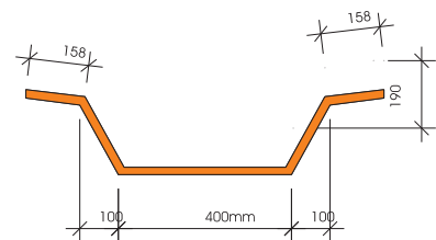
TYPE2 VALLEY GUTTER
