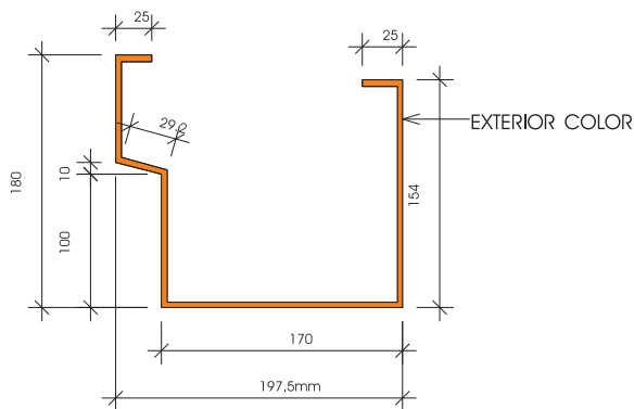
EAVE GUTTER
