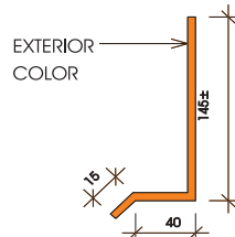
DRIP TRIM FOR PARTIALLY OPEN WALLS
