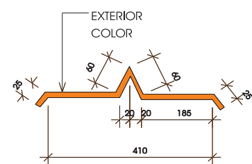
EXPANSION JOINT TRIM FOR ROOF AND WALLS
