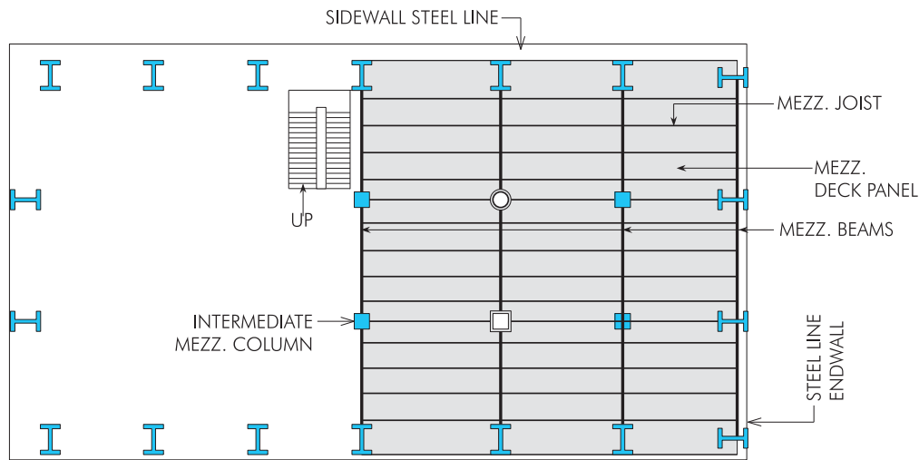
Column & Beam arrangement
