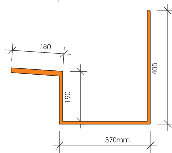
TYPE1 VALLEY GUTTER
