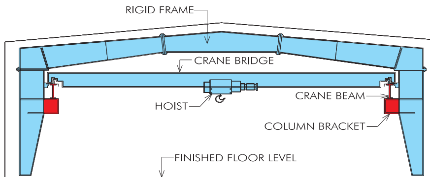
Top Running Crane
