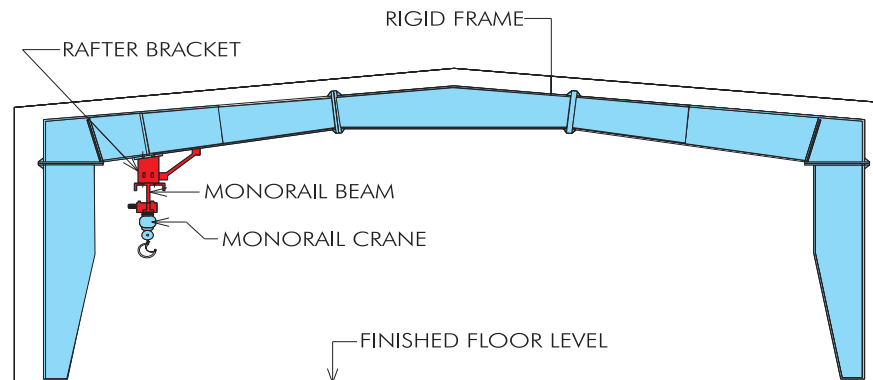
Monorail Crane
