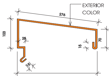
CAP FLASHING
