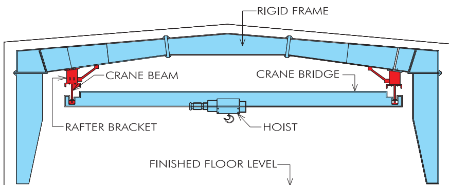
Underhung Crane
