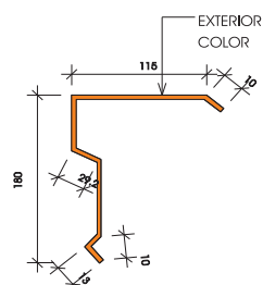
OASIS GABLE TRIM AT ENDWALLS ONLY
