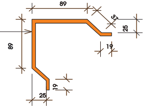
OUTSIDE CORNER TRIM AT INTERSECTION OF ENDWALL AND SIDEWALL
